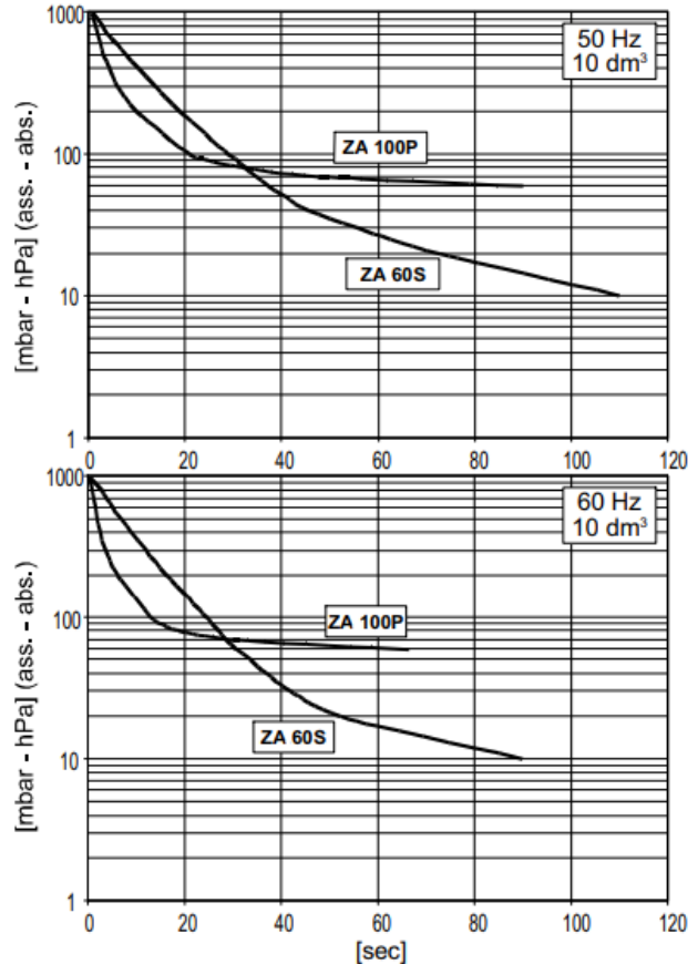
NOTE: Curves refers to 1013mbar (abs.) pression and 20°C temp. (tolerance ±10%).
